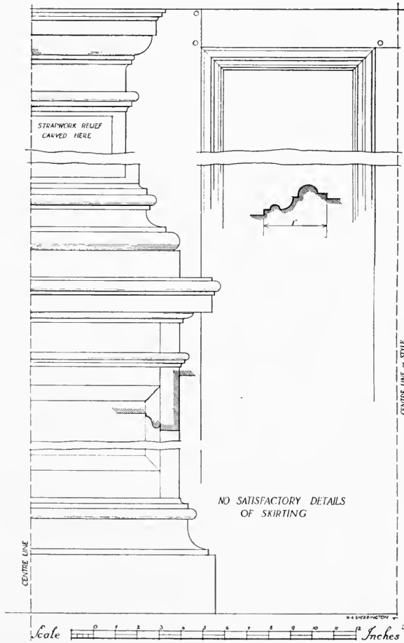
Measured drawing of section of Pilaster (see p. 11).
